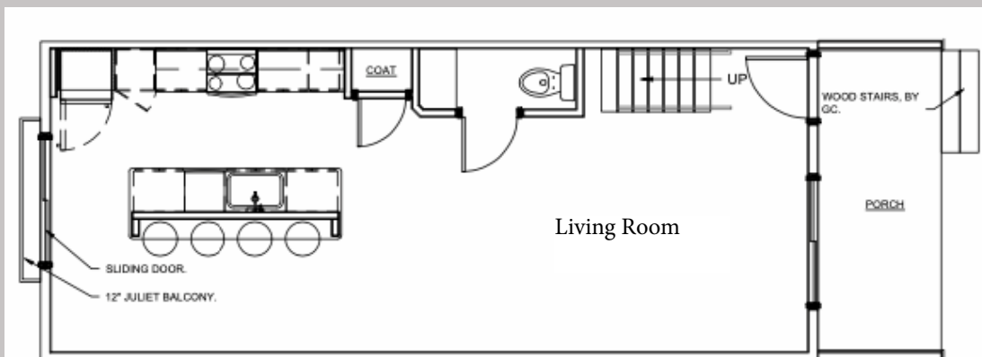
Ground Floor - 692 SF
